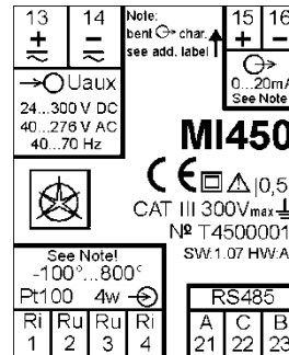
Picture 6b: Example of label for transducer with bent characteristic
