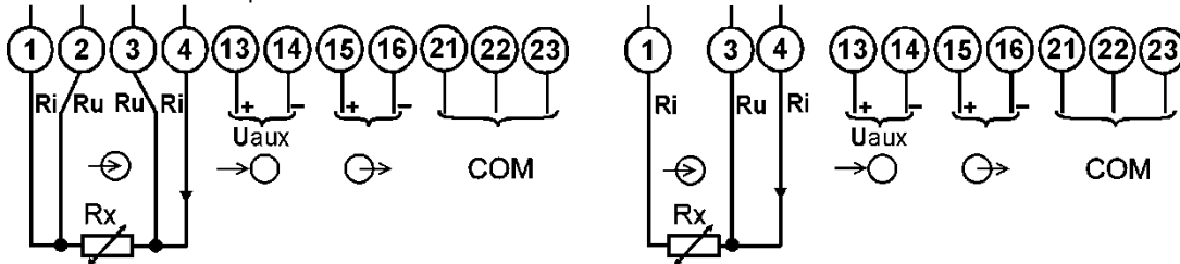
Picture 7a: Connection diagram 4-wire
