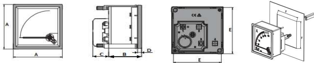
Moving Coil meter 4-20mA DC
