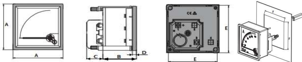
Moving Coil meter Direct Ammeter DC
