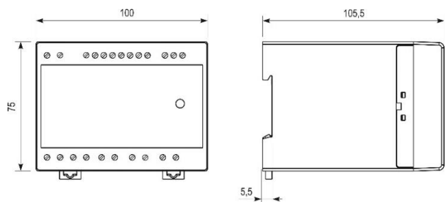
Dimensions for iMT440.
